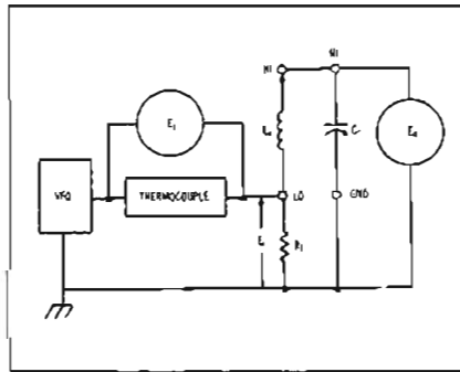
Figure 2. Q Meter.
