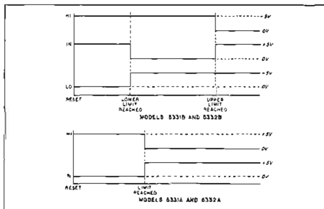
Figure 1. Control line outputs in MANUAL and HOLD modes.
