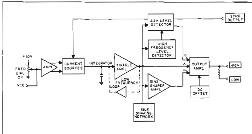
Figure 1. Block diagram of 3310A Function Generator.
