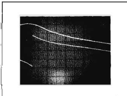
Figure 7. Amplifier Voltage Gain—This open-loop video amplifier can be analyzed for gain, bandwidth, and distortion (phase shift) while still in the breadboard stage with the passive voltage probes. Gain is 50 dB at low frequencies, dropping down to about 27 dB at 50 MHz. Amplitude is 10 dB/division; phase 100°/division. Phase shift is quite linear above 20 MHz.
