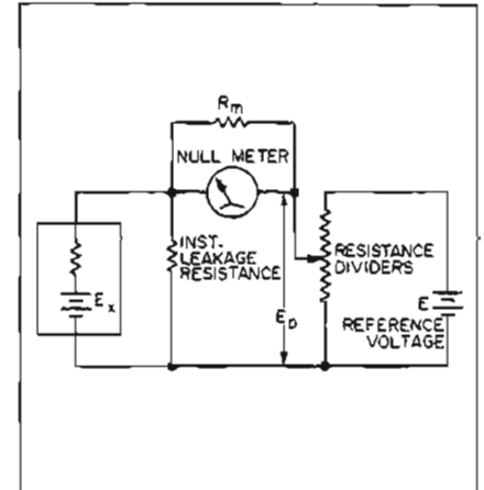
Figure 6. Classic differential voltage measurement.
