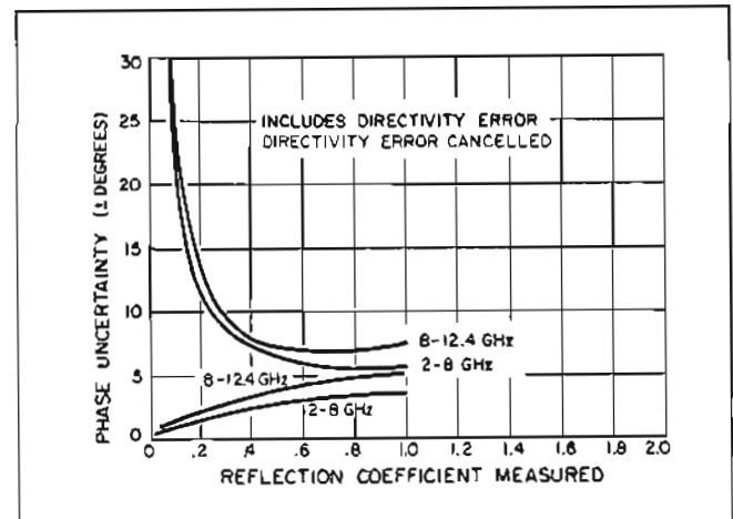
Phase uncertainty including coupler directivity and when directivity is cancelled using a sliding load.
