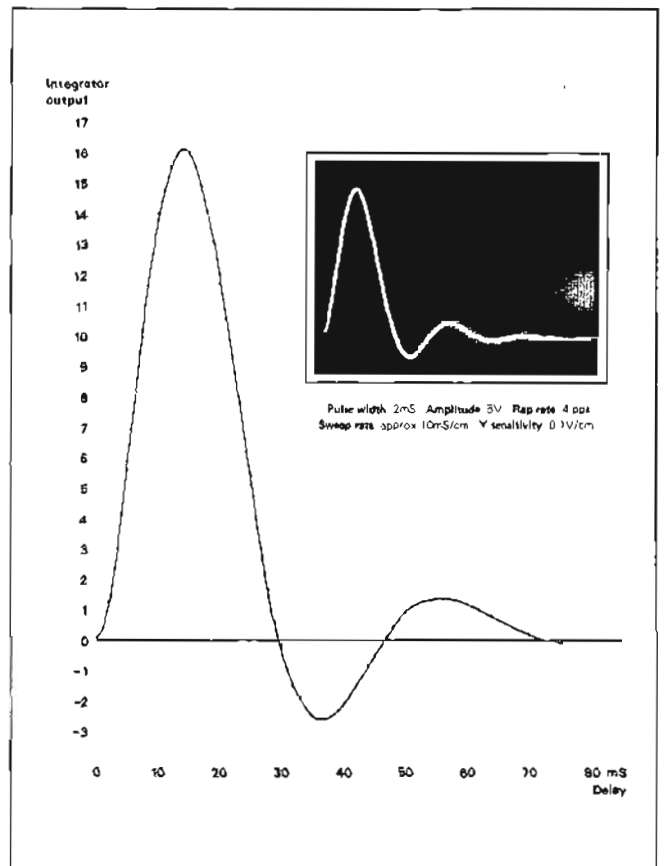
Impulse response of LC filter measured using 3722A option H01. Photo inset shows filter's response to a 2 ms pulse.
