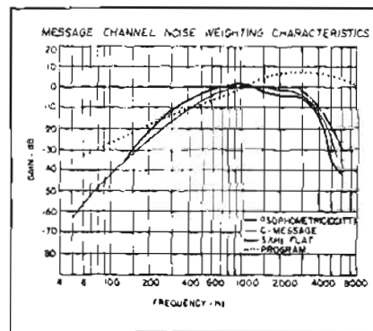
Figure 1. Noise weighting curves.
