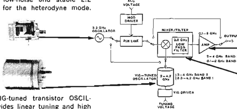
8699B Block Diagram
