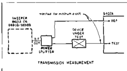
Figure 5. Transmission Measurement
