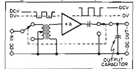
Figure 3. Modulated amplifier.
