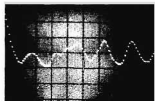
Autocorrelation of background noise in office area. Shows periodic component due to ventilation fan, normally inaudible. Timescale 1 ms/mm.
