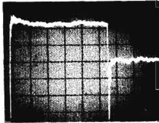
Impedance Mismatch: Reflection caused by cables of different impedance. With the vertical calibrated in .02 \text{ p/div} and the first cable known to be 75\Omega , the second cable is quickly found to be 69\Omega using the TDR slide rule. From scope readout, the mismatch is located 55 ft down the 75\Omega cable.
