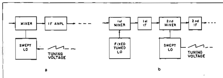
Figure 2. Two Methods of Obtaining Swept-Frequency Capability. a. Spectrum Analyzer using swept first LO. b. Spectrum Analyzer using swept second LO.
