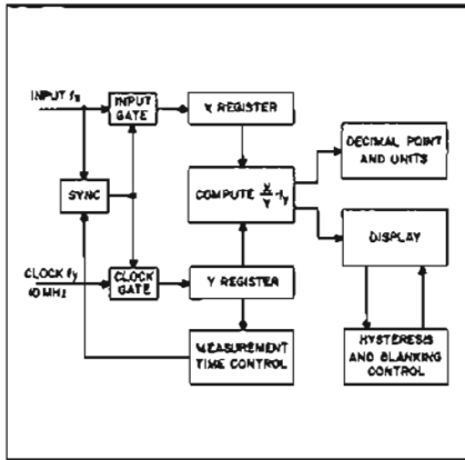
Figure 10. 5323A Automatic Counter. Computing circuits divide the number of input cycles (X) by the number of clock periods (Y) and multiply by f_c = 10^7 to find the unknown frequency f_x . Other IC's determine the measurement units, position the decimal point, blank insignificant digits, and apply hysteresis to prevent display jitter.
