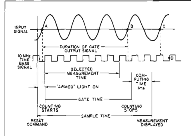
Figure 2. The Measurement Cycle.
