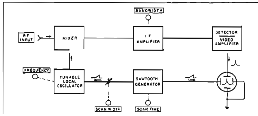
Figure 1. Simplified Spectrum Analyzer of the Swept-Receiver Design.
