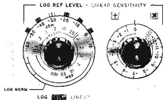
Figure 3. Settings of the INPUT ATTENUATOR and LOG REFERENCE LEVEL controls determine the scale factor for absolute amplitude calibration. Here, LOG is selected and the "+" lamp lights to indicate that LOG REFERENCE LEVEL is the sum of the black color-coded dial readings; i.e., LOG REF = -30 dBm + 0 dBm = -30 dBm.
