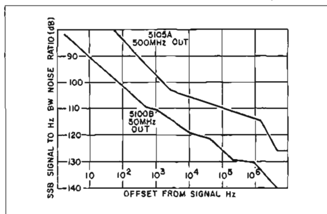
Figure 2. Composite phase noise plot for Hewlett-Packard synthesizer.
