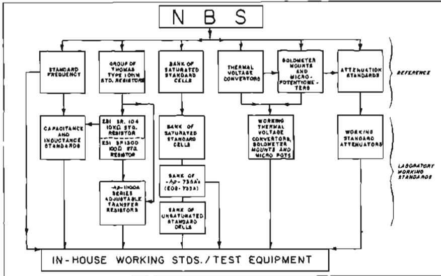
Figure 1. HP instrument traceability to NBS.
