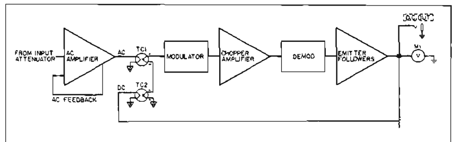
Figure 6. True rms-responding voltmeter.
