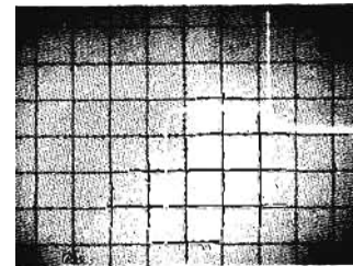
System Profile: Reflection pattern as seen by looking down a transmission system. The pattern reveals a low impedance cable (off screen) connected to a 69\Omega cable. 27 ft from the connector is an inductive defect; 20 ft farther along is a capacitive defect from a pinched cable; 8 ft from the pinch is a 67\Omega termination.
