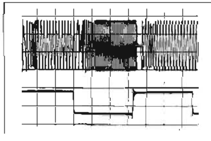
Figure 1. Switching speed, Model 5103A: 1.2 MHz to 2.7 MHz, 30 kHz switching rate. 5 \mu s/cm, 10 MHz Range.
