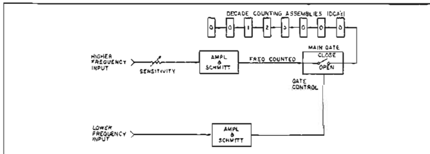
Figure 5. Ratio measurement. Function switch set to Period and time base switch to Ext. Lower frequency controls gate, while higher frequency replaces time base as counted frequency.
