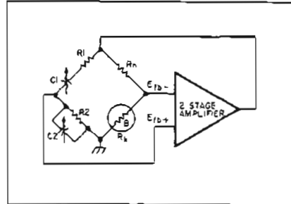
Figure 6. Basic HP Wien bridge RC oscillator circuit.
