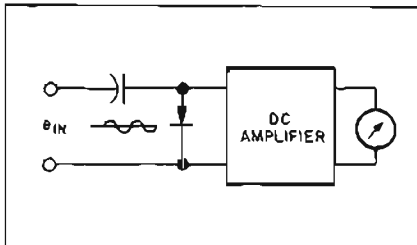
Figure 5. Peak-responding voltmeter.
