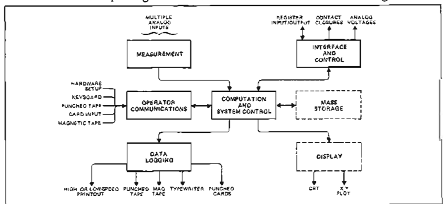
Hardware and computer-controlled data acquisition system composite block diagram.
