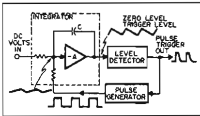
Figure 4. Voltage-to-frequency conversion.
