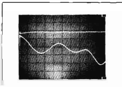
Figure 6b. Sweep is 1 - 40 MHz (4 MHz/div.) and amplitude resolution is 0.25 dB/div. Insertion loss and passband ripple are measured to an accuracy of several hundredths of dB.
