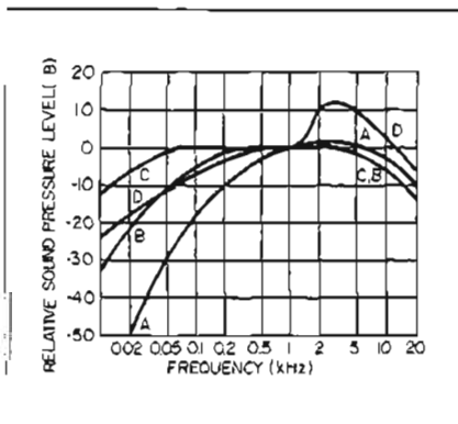
Figure 2. Frequency response curves.
