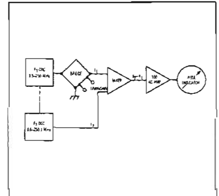
Figure 3. RX Meter.
