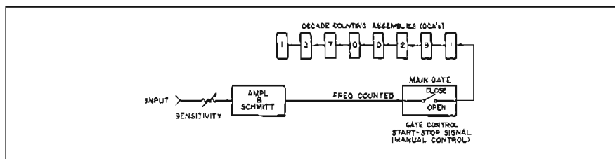
Figure 1. Function switch set to manual Start and Stop for totalizing.
