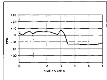
Figure 3. 6 month stability of a 745A reference supply.
