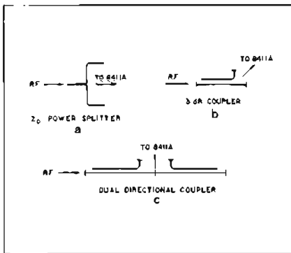
Figure 16. Reference and test channels for the network analyzer may be obtained using various methods such as a) power splitters, b) 3-dB couplers, c) dual directional or back-to-back couplers. The second coupler in c would be turned around for transmission measurements.
