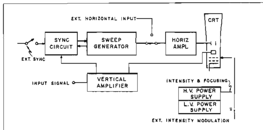
Figure 2. Oscilloscope block diagram.
