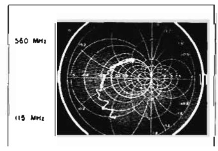
Figure 22. Swept-frequency display of impedance of a tunnel diode when it is biased in the negative impedance region.
