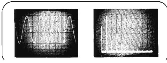
Harmonic Distortion in Time-Domain—Hardly Visible
