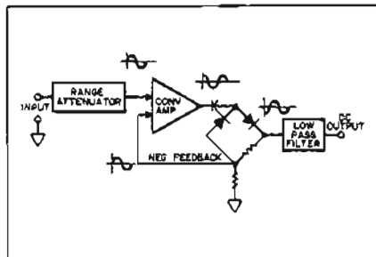
Figure 10. Typical ac/dc converter.
