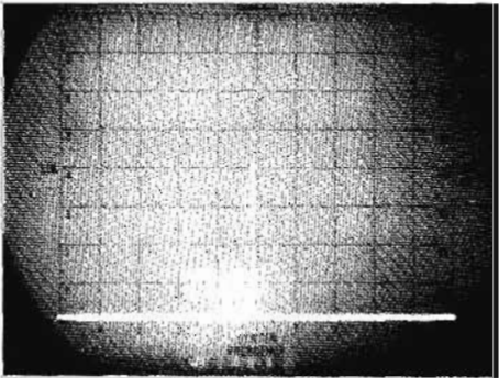
Figure 2. Signal selected by the marker from the comb of Figure 1. Signal amplitude is 38 dB below REF, and the display is LOG (power). The LOG REFERENCE LEVEL (from fig. 3) is -30 dBm, therefore amplitude is -68 dBm.
