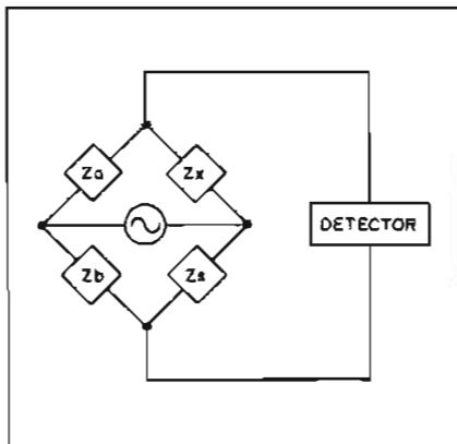
Figure 1. Generalized Bridge Circuit
