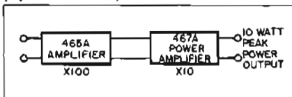
Figure 1. Cascading the HP 467A Power Amplifier with the HP 465A Amplifier results in a stable 60 dB amplifier with 10 M \Omega input impedance and 10 W peak-power output.
