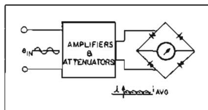
Figure 3. Average-responding voltmeter.
