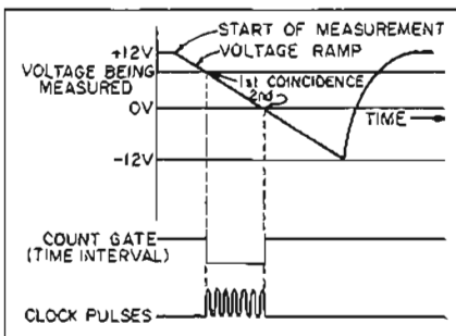
Figure 1. Voltage-to-time conversion.
