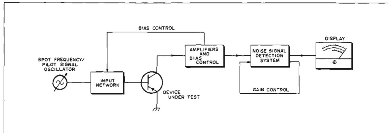
Figure 3. 4470A Basic Block Diagram
