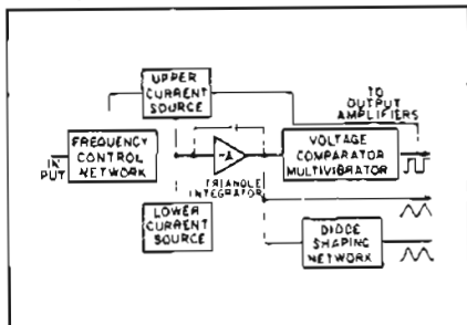
Figure 2. 3300A Function Generator.
