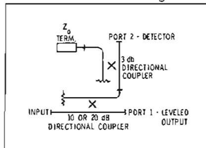
Figure 2. Super leveling with back-to-back waveguide coupler arrangement for extremely flat output.
