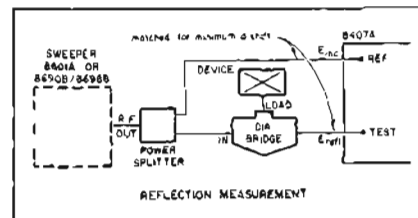
Figure 8. Reflection Measurement.
