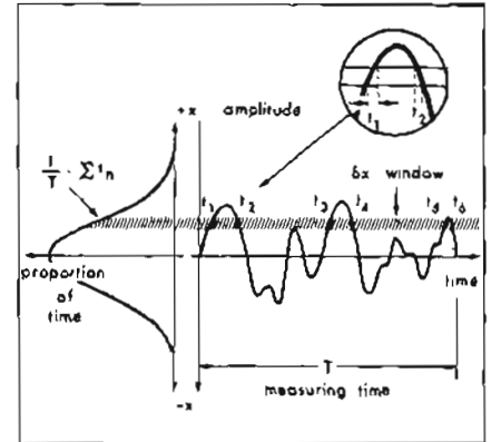
Figure 4. Measuring pdf of random signal.
