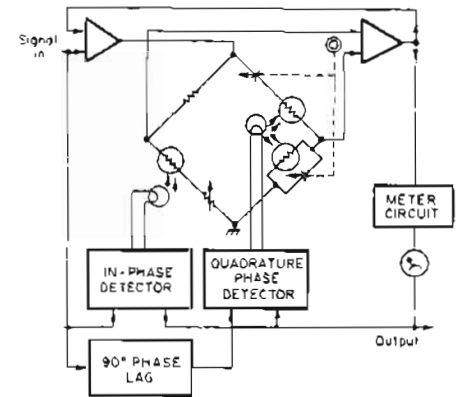
Figure 2. Rejection amplifier with automatic nulling circuitry. Phase detectors sense bridge unbalance and control intensity of lamps to change resistance of photoconductors, thus adjusting bridge to reject fundamental frequency of input signal.
