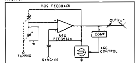
Figure 8. Block diagram of the 204C Oscillator.
