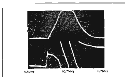
Figure 3. Phase and amplitude response of an LC filter displayed on an oscilloscope.
