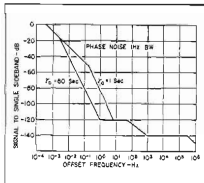
Figure 2. 5061A phase noise.
