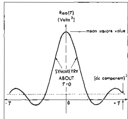
Figure 2. Autocorrelation function of random signal.
