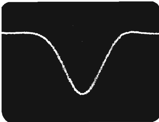
CRT display using Model 1815A/1817A/1106A TDR system slows the reflection from HP Model 8748 Susceptance Standard set at 1 pF equivalent capacitive discontinuity. Scale: 20 ps/div horizontal, 0.1 p/div vertical.
