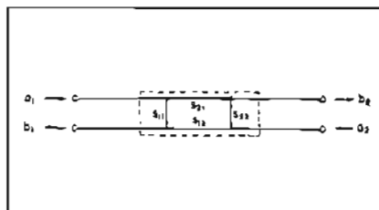
Figure 25. S-parameter representation of a two-port microwave device.
