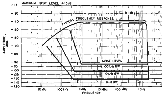
Figure 1. Noise level vs. Input Frequency.
