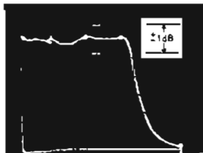
Figure 1. Frequency response curve of HP 461A. Markers shown from left to right are: 50, 100, 150 and 200 MHz. Gain control is set in 20 or 40 dB position.
