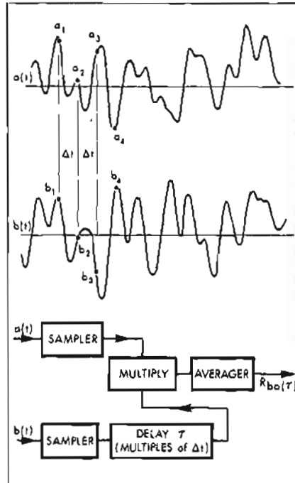
Figure 3. Computing crosscorrelation function.
