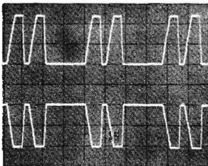
Figure 1. (a) Separate output in double pulse mode. (b) Combined and separate non-simultaneous outputs. (c) A/B gating of combined and separate outputs.
