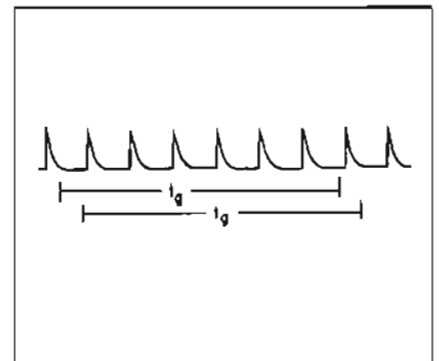
Figure 8. An error of \pm 1 count can occur because gate may open and close between input pulses. With gate open for upper t_g interval, 6 counts occur; 7 counts occur for lower interval.
