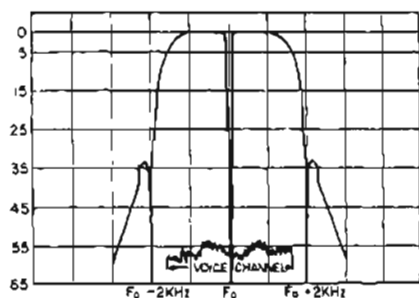
Figure 4. Bandpass for the 312A Selective Voltmeter.
