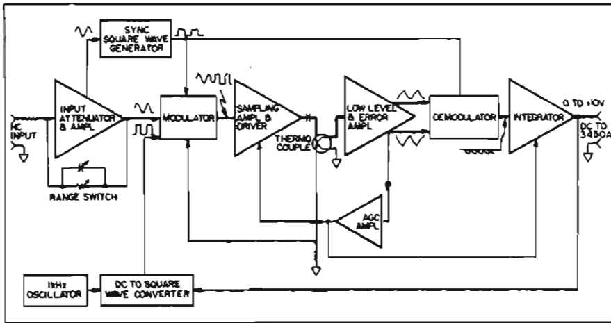
Figure 8. Ac-dc converter for the 3450A.
